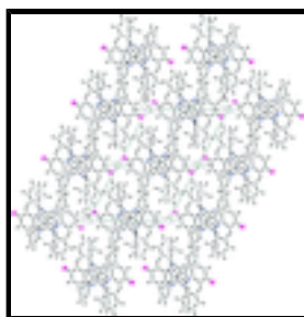
Fig. 2. The unit cell contents of the title compound in projection along [010]. The solvent molecules (benzene) are present at the centres of symmetry 0,0,0 and 0,1/2,1/2.
