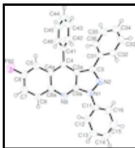
Fig. 1. The conformation of the 6-fluoro-1,3,4-triphenyl-1 H -pyrazolo[3,4- b ]quinoline molecule with the atom numbering scheme. Displacement ellipsoids are drawn at the 50% probability level and H atoms are shown as small spheres of arbitrary radii.
